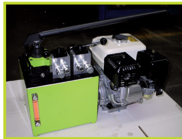
10 litres Petrol powerpack with manual pump, 2 valves and by-pass.
